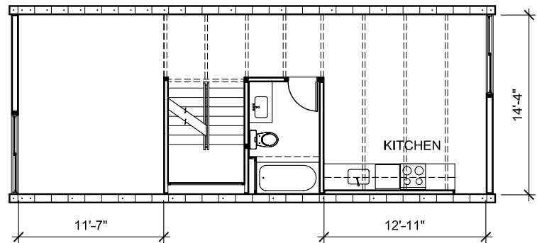
Second Floor
