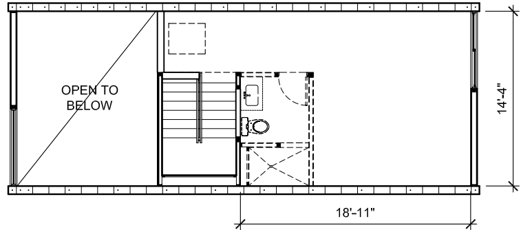
Third Floor
